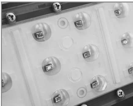
LED'S AND OPTICS DETAILS
